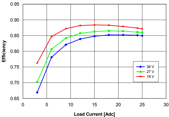
Fig. 16: Efficiency vs. load current and input voltage for converter mounted horizontally with air flowing from pin 3 to pin 4 at a rate of 300 LFM (1.5 m/s) and T_a = 25\text{ }^\circ\text{C} .
