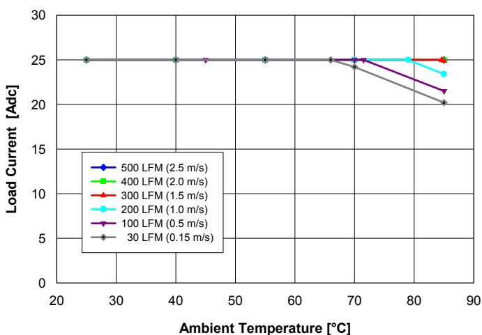
Fig. 1: Available load current vs. ambient air temperature and air-flow rates for Q24S25020 converter mounted vertically with air flowing from pin 3 to pin 1, MOSFET temperature \leq 120 °C, V_{in} = 27 V.
