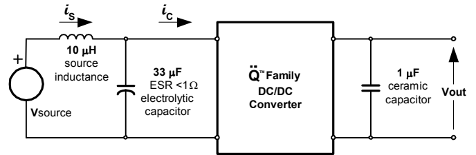
Fig. 23: Test setup for measuring input reflected ripple currents, i_c and i_s .
